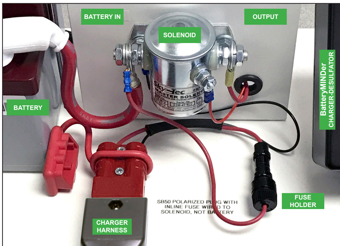
Figure 1. Simplified example of connection to battery solenoid. For more examples, see www.audioauthority.com/bmaik .
